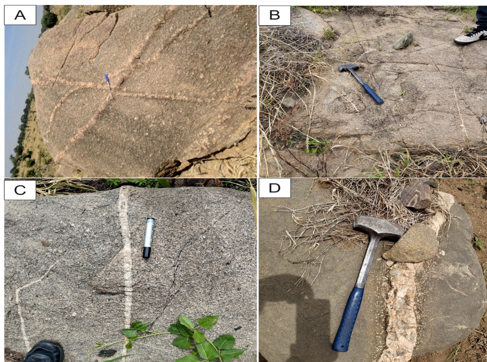
Figure 6: Quartzo-feldspathic veins (a) and numerous joints (b) in porphyritic biotite granite; (c) quartz veins in the equigranular granite; (d) Quartzo-feldspathic veins in the intermediate rock (monzodiorite).
