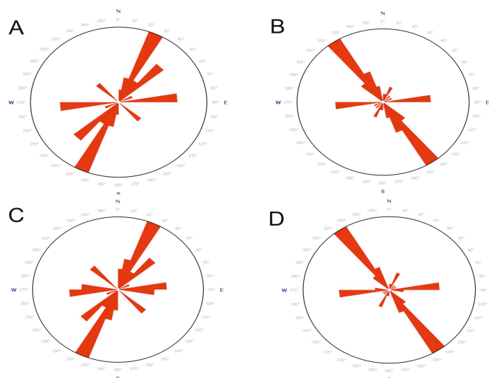
Figure 7. Rose Plot for veins (a) and joints (b) for porphyritic biotite granite; rose plot of veins (c) and joints (d) for equigranular granite. Showing NE-SW as the dominant trend for the veins; and NW-SE as the major trend for the joints.
