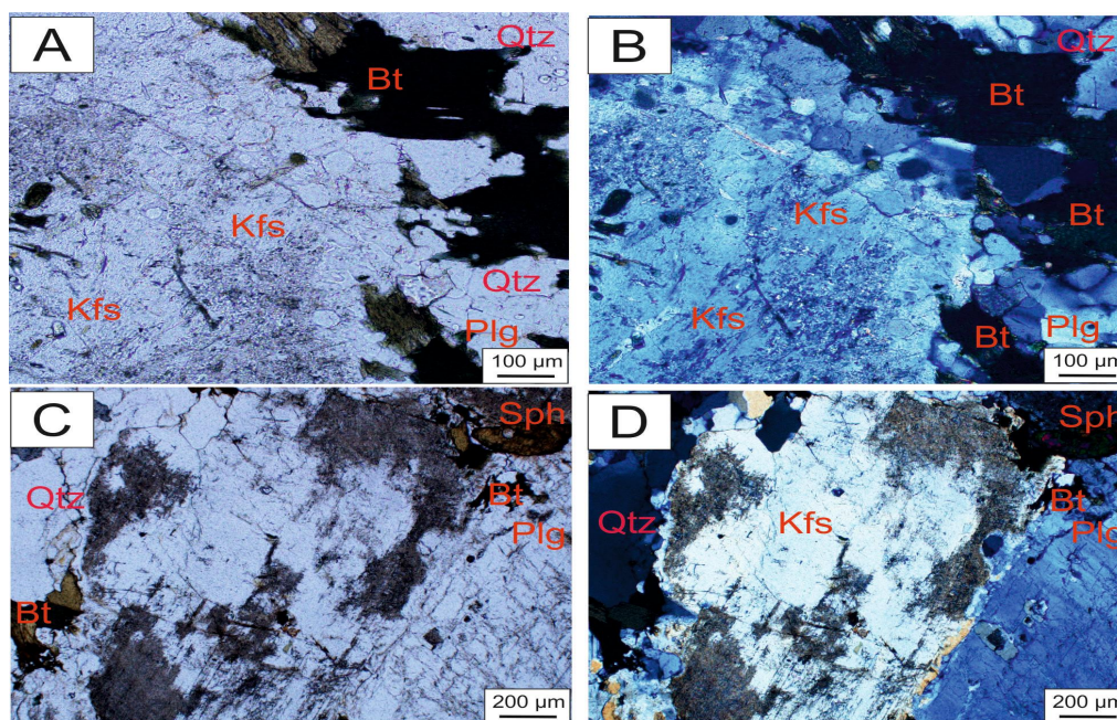
Figure 4: Photomicrograph of porphyritic biotite granite under PPL (a) and XPL (b) depicting the phenocryst of microcline; Photomicrograph of equigranular granite under PPL (a) and XPL (b) showing the nearly equal crystal size with sphene (titanite) grains as accessory. Qtz: Quartz; Bt: Biotite; Plg: Plagioclase; Kfs: K-feldspar; Sph: Sphene.
