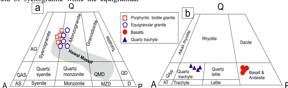
Figure 8: (a) IUGS classification of plutonic rocks based upon modal mineralogy After Le Bas and Streckeisen (1991); (b) IUGS classification of volcanic rock based on modal mineralogy (Le Bas and Streckeisen 1991). A = alkali feldspar, P = plagioclase, Q = quartz.
