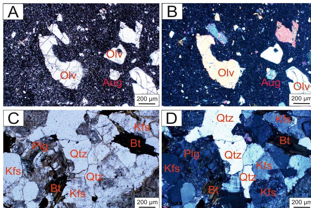
Figure 5: Photomicrograph of basalt under PPL (a) and XPL (b) showing phenocryst of olivine and matrix made up of plagioclase laths and iron oxide; photomicrograph of trachyte under PPL (a) and XPL (b) showing zoned plagioclase and flakes of biotite. Plg: Plagioclase, Oliv: Olivine, Aug: Augite, Opq: Opaque; Kfs: K-feldspar
