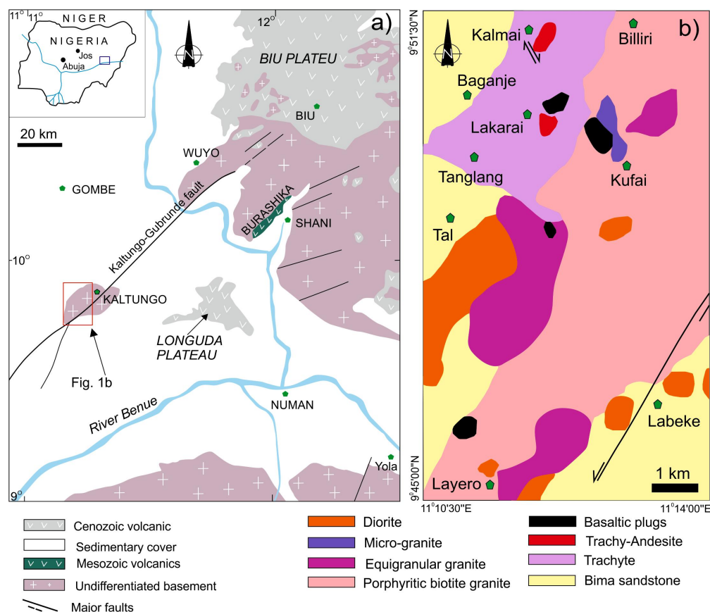
Figure 1: (a) Regional geological map of Upper Benue Valley showing the Kaltungo-Gubrunde inliers (modified from Maurin et al., 1986); (b) Geological map of Kufai and environs (Western Kaltungo inlier), modified from Tabale et al., (2017).
